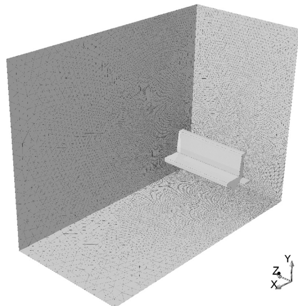
Fig. 10. CFD model.
